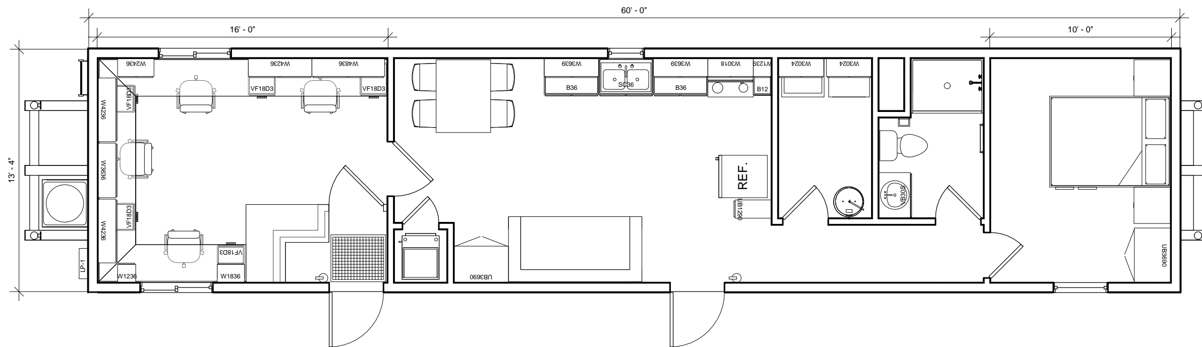
1 A000 Sales 3/16" = 1'-0"
