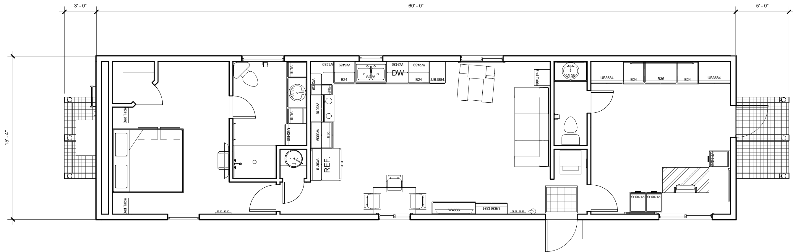
1 SALES PLAN 3/16" = 1'-0"
