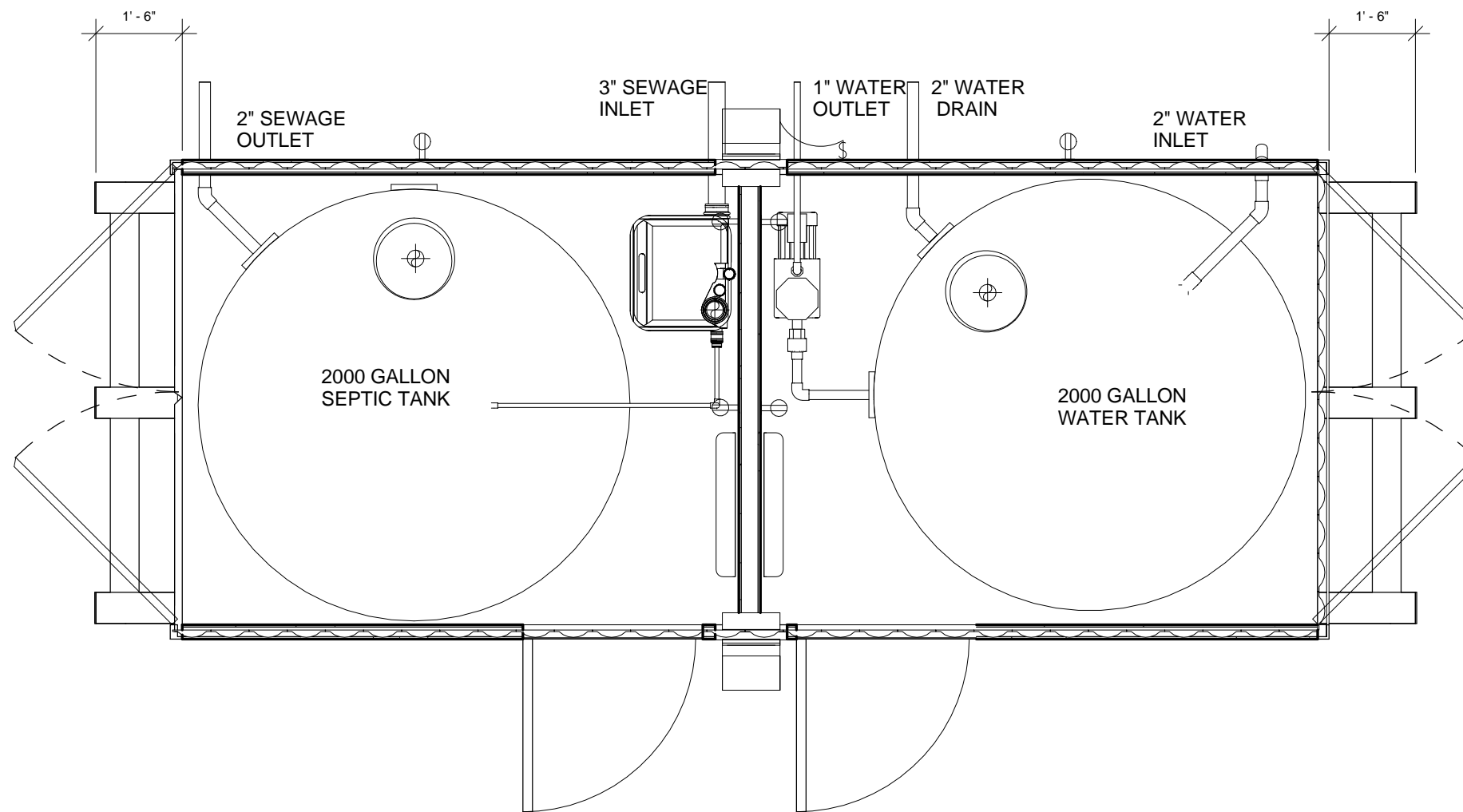
1 SALES PLAN 3/8" = 1'-0"
