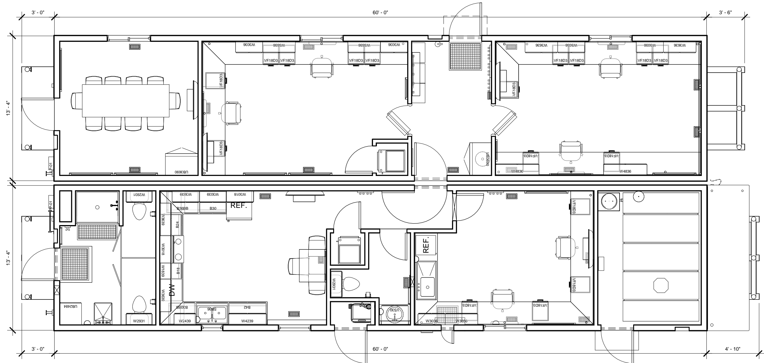
1 A000 Sales 3/16" = 1'-0"
